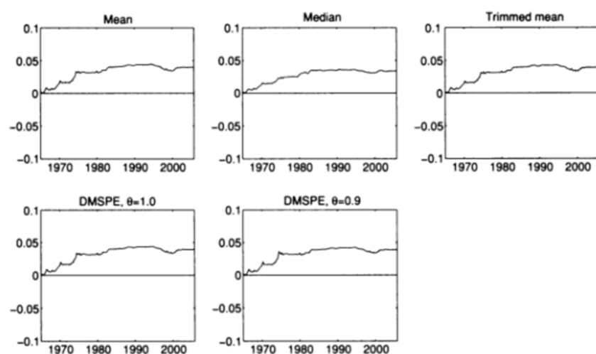
Figure 2 Cumulative square prediction error for the historical average benchmark forecasting model minus the cumulative square prediction error for the combination forecasting model, 1965:1-2005:4 The dotted (solid) line corresponds to combination forecasts based on individual model forecasts that (do not) impose Campbell and Thompson (2008) restrictions.
