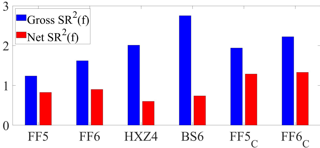
Figure 1: Maximum squared Sharpe ratios of factor models. This figure presents maximum squared Sharpe ratios from the factors in the models listed on the x-axis. The blue columns, ‘Gross SR^2(f) ’, use factor returns that ignore transaction costs. The red columns, ‘Net SR^2(f) ’, use factor returns that account for transaction costs. The sample period is January 1972 to December 2017.
