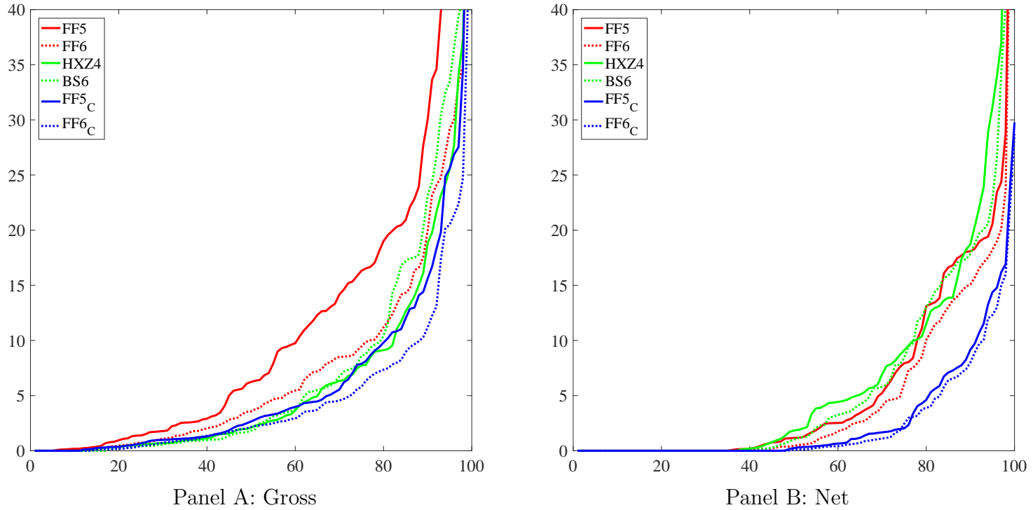
Figure 2: Frontier expansion (squared Sharpe ratio improvement) from adding anomalies to asset-pricing models. For each asset-pricing model we consider, M , and each of the 120 anomalies, A , described in Section 4, we compute the maximum ex-post squared Sharpe ratio attainable from the model's factors, SR^2(M) , along with the maximum squared Sharpe ratio attainable from the model's factors and the anomaly, SR^2(M, A) . We then compute the squared Sharpe ratio improvement, \% \Delta SR(M, A) = SR^2(M, A) / SR^2(M) - 1 . This figure depicts plots of the percentiles from the distribution of the 120 \% \Delta SR(M, A) for each model specified by the plot legend. Panel A (B) ignores (accounts for) transaction costs. For ease of visualization, the y-axes are truncated at 40%.
