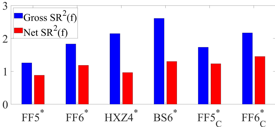
Figure 3: Maximum squared Sharpe ratios of cost-mitigated factor models. This figure presents maximum squared Sharpe ratios from the factors in the models listed on the x-axis. The blue columns, ‘Gross SR^2(f) ’, use factor returns that ignore transaction costs. The red columns, ‘Net SR^2(f) ’, use factor returns that account for transaction costs. The factors are all versions that use the 20% banding cost-mitigation strategy described in Section 5. The sample period is January 1972 to December 2017.
